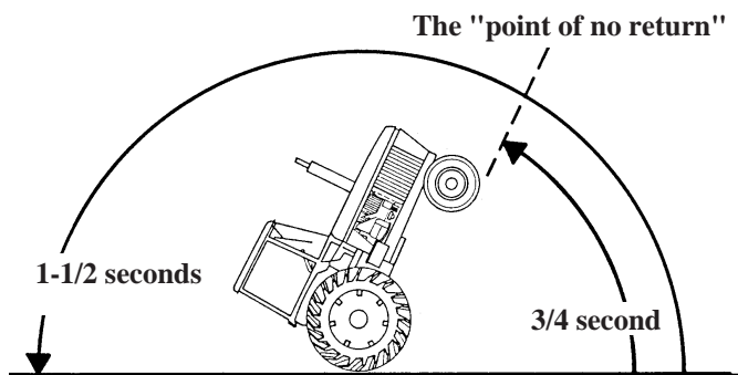
Figure 3. The "point of no return" during a rear turnover may be reached in 3/4 of a second.
